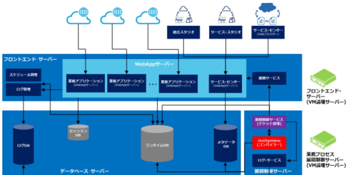
図 1 1 OutSystems Platform
